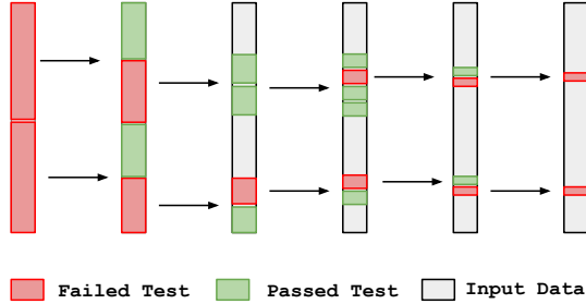
Figure 4: Automated fault localization using Delta Debugging
