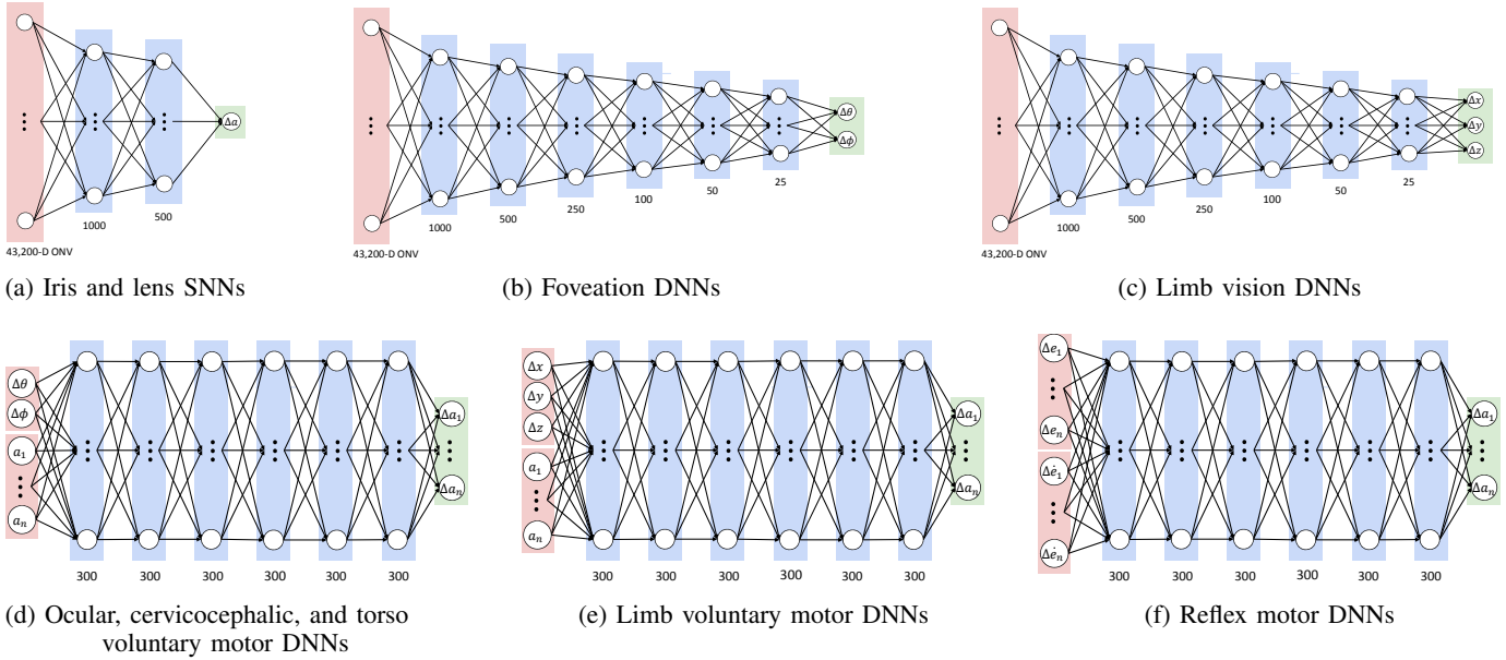
Fig. 3: Network architectures of the (a)–(c) vision SNNs and DNNs, and (d)–(f) motor DNNs.
