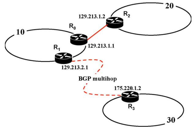
Fig. 3. Configuring remote BGP peering. R_0 and R_2 are physically directly connected, while R_1 and R_3 are not.
