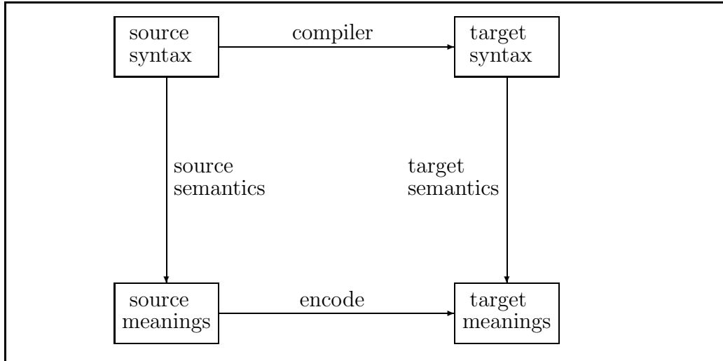
Figure 2: Compiler correctness.
