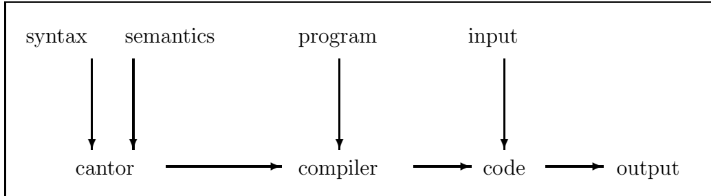
Figure 4: The Cantor system.
