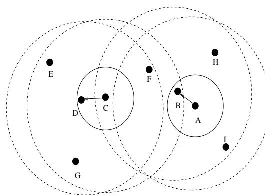
Fig. 2. Motivation for Power Control in Collision Avoidance-based Medium Access. For the given placement of nodes, in a traditional collision avoidance-based MAC protocol, if C is sending to D then A could not send to B since B would hear the RTS from C and sense the ongoing transmission. However, if C reduced its transmission power such that it would be just enough for D to capture its signal then other nodes in the region (e.g. A) could also proceed with their transmission. Such a protocol would allow for a tighter packing of source destination pairs within a network environment, thereby improving the spectral reuse.
