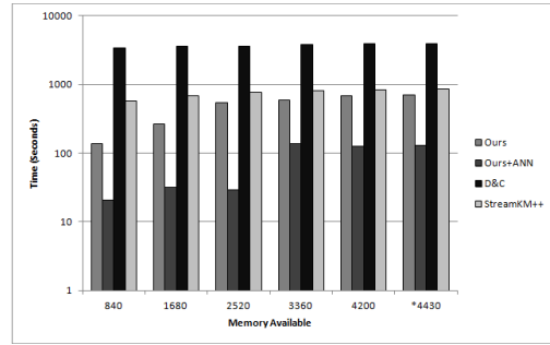
Figure 2: Census Data, k=8, time
