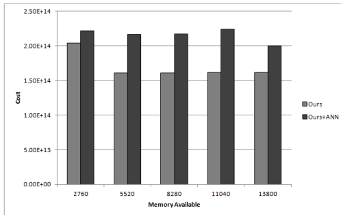
Figure 7: BigCross Data, k=24, cost
