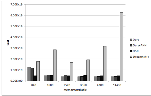
Figure 1: Census Data, k=8, cost
