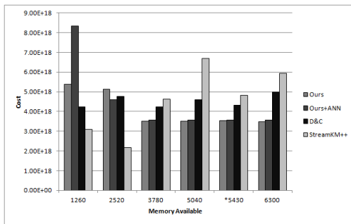
Figure 3: Census Data, k=12, cost
