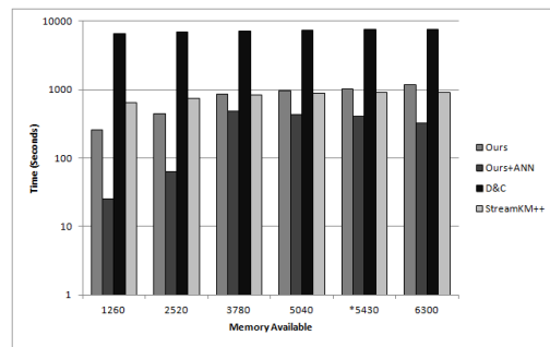
Figure 4: Census Data, k=12, time
