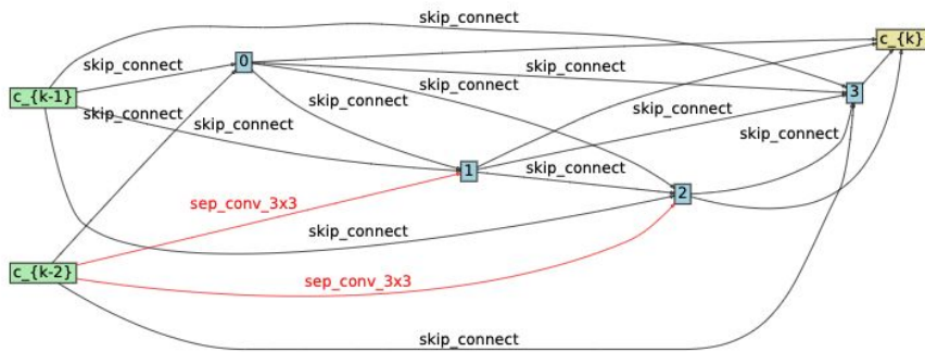
Magnitude-base selection
