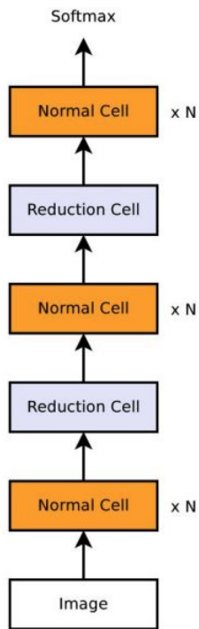
CIFAR10 Architecture
