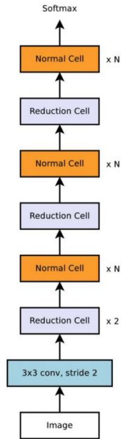
ImageNet Architecture
