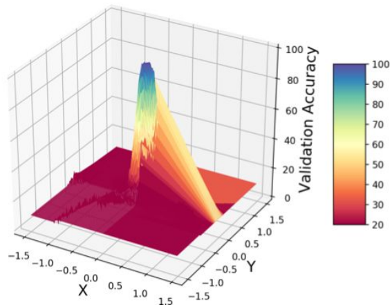
(a) DARTS
