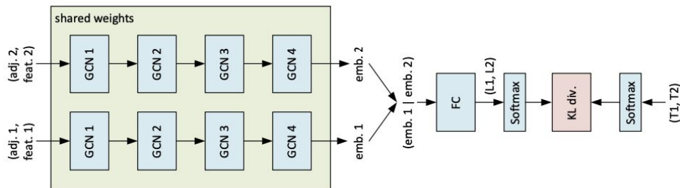
Siamese ranker with GCN encoder (Dudziak et al., 2020)
