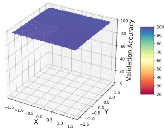
(c) SDARTS-ADV
