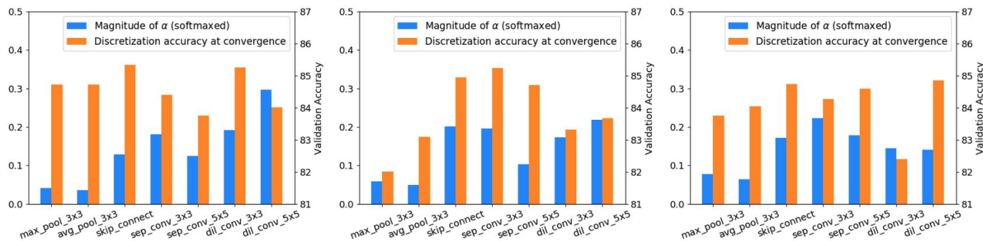
Figure: Magnitude of \alpha vs Accuracy after choosing one operation
