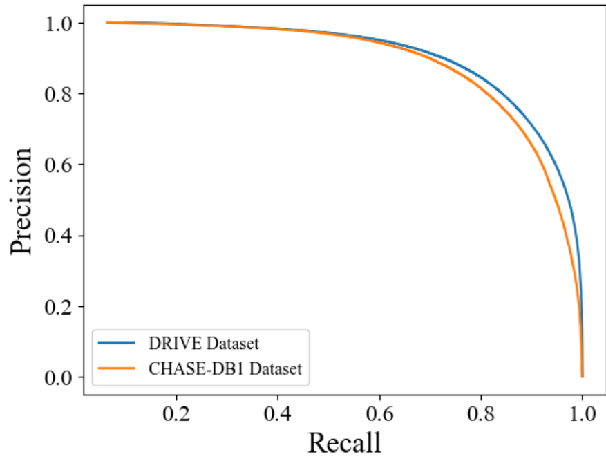
Figure 5.1: Precision-Recall curves for our model’s segmentation performance on the DRIVE and CHASE-DB1 datasets.
