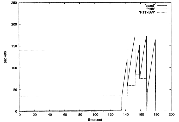
Fig. 5. Example of TCP congestion window; max MAC retr = 2.
