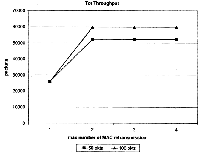
Fig. 8. FTP total throughput with different MAC queue sizes; distance from the AP = 5m, shadowing deviation = 9.
