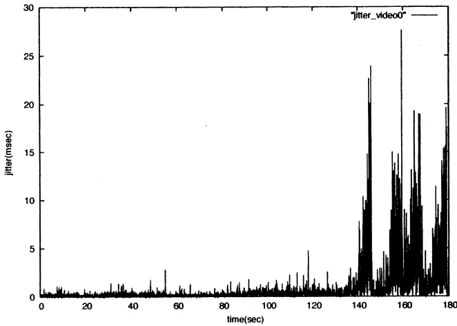
Fig. 2. Example of movie streaming jitter.
