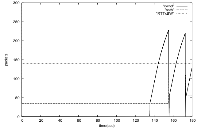
Figure 3. Measured TCP congestion window when the regular TCP NewReno and IEEE 802.11g are employed.
