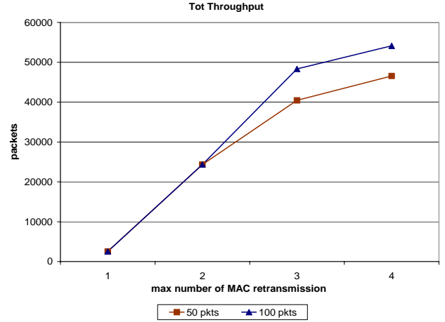
Figure 5. FTP total throughput with different MAC buffer sizes; user-AP distance = 10m, shadowing deviation = 9.
