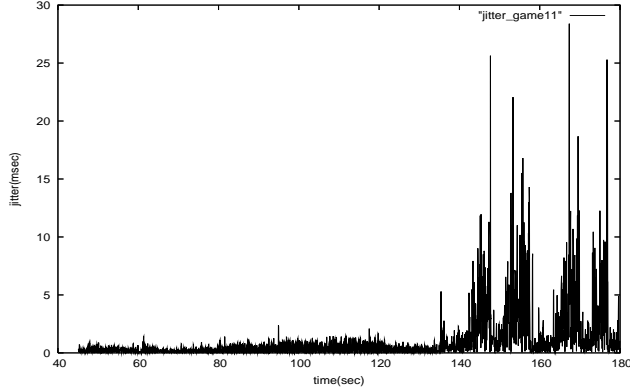
Figure 7. Measured online game jitter with max 3 retransmissions at the IEEE 802.11g MAC layer; from 135s, a regular TCP NewReno flow is competing for the channel.
