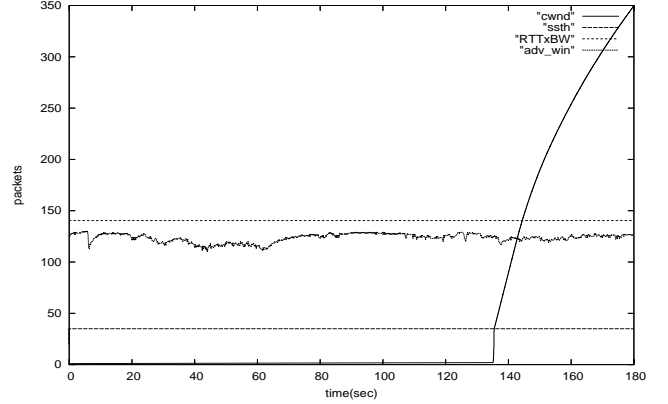
Figure 9. Measured congestion window and advertised window of a SAP-LAW flow with C = 18 Mbps; regular IEEE 802.11g employed.
