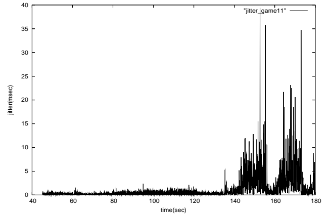
Figure 4. Measured online game jitter with regular IEEE 802.11g employed; from 135s, a regular TCP NewReno flow is competing for the channel.
