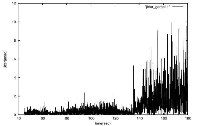
Figure 10. Online game jitter with regular IEEE 802.11g employed; from 135s, a SAP-LAW flow with C = 18 Mbps is competing for the channel.
