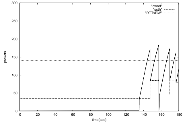
Figure 6. Measured TCP NewReno congestion window with max 3 retransmissions at the IEEE 802.11g MAC layer.
