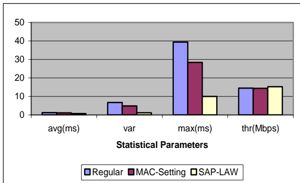
Figure 11. Statistical values of the online game stream for the compared schemes.
