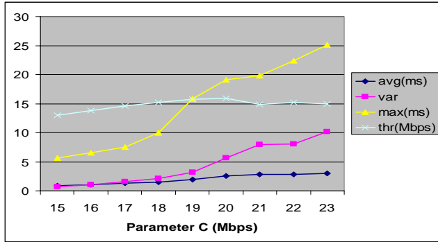
Figure 8. Throughput achieved by the FTP flow and jitter statistics of the game flow when employing SAP-LAW.
