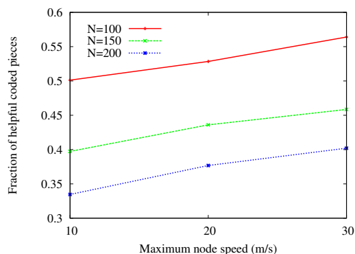
Figure 6: Helpfulness as a function of node speed
