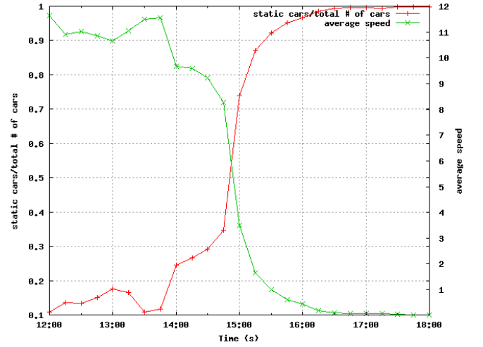
Fig. 8. Average car speed and fraction of static cars, between 12:00PM and 6:00PM, in the 1 x 2 km Portland area.
