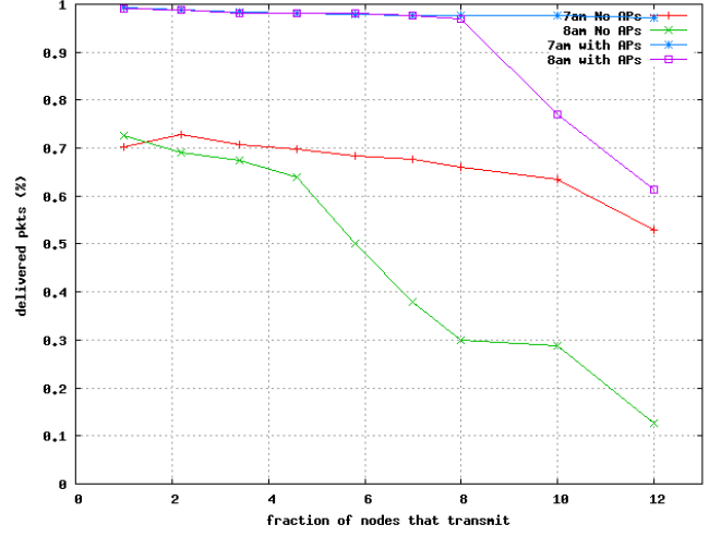
Fig. 3. 7AM and 8AM delivery ratio, with and without infrastructure, using the RWP model, as the number of sources increases.
