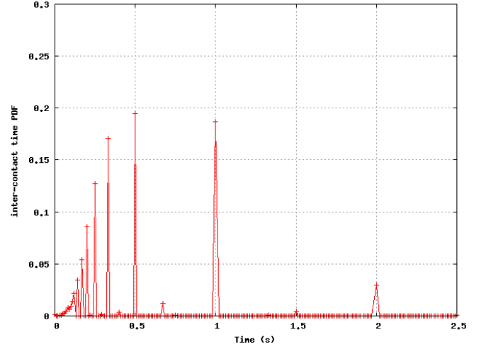
Fig. 6. Inter-contact time, in TRANSIMS mobility traces, at 8AM.
