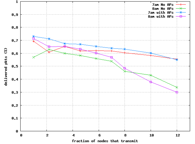
Fig. 4. 7AM and 8AM delivery ratio, with and without infrastructure, using the CORSIM mobility traces generated introducing traffic lights, as the number of sources increases.
