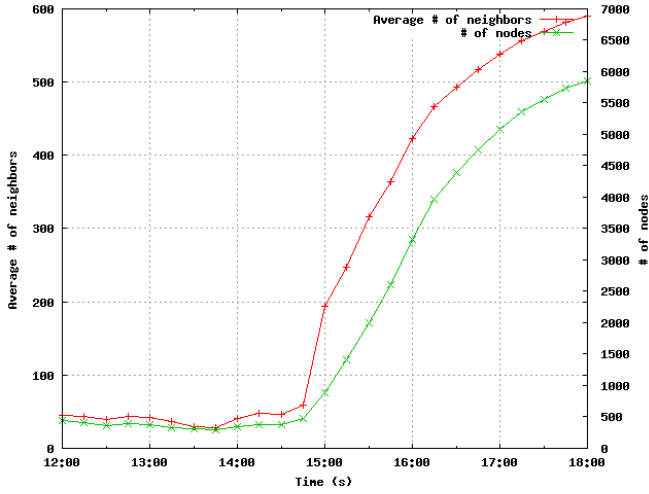
Fig. 7. Total number of cars and average number of neighbors per car, between 12:00PM and 6:00PM, in the 1 x 2 km Portland area.
