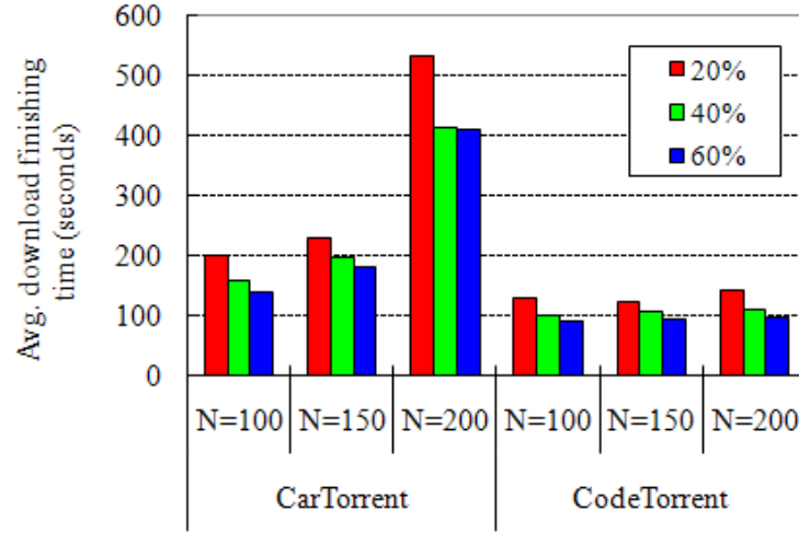
Fig. 8. Impact of popularity on average download delay
