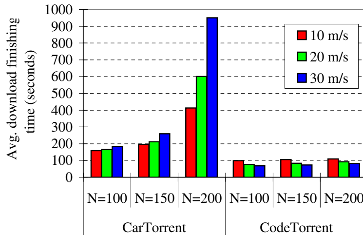
Fig. 4. Impact of mobility on average download delay
