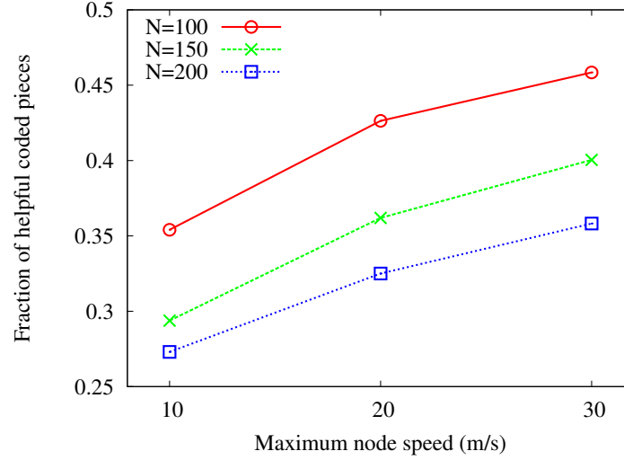
Fig. 6. Helpfulness as function of node speed
