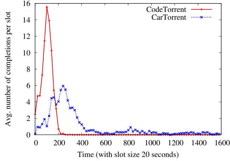
Fig. 2. Histogram of download delays
