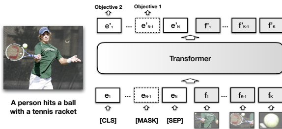
Figure 2: The architecture of VisualBERT. Image regions and language are combined with a Transformer to allow the self-attention to discover implicit alignments between language and vision. It is pre-trained with a masked language modeling (Objective 1), and sentence-image prediction task (Objective 2), on caption data and then fine-tuned for different tasks.
