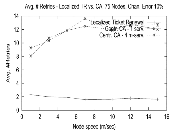
Fig. 7. Average number of retries versus node speed, ticket renewal with a 10% channel error rate.
