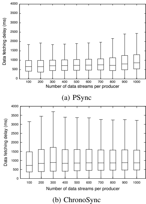
Fig. 16: Data Fetching Delay in Full-Data Synchronization
