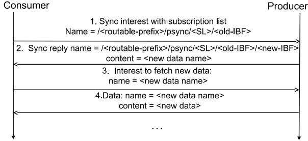
Fig. 8: Sync Phase in PSync
