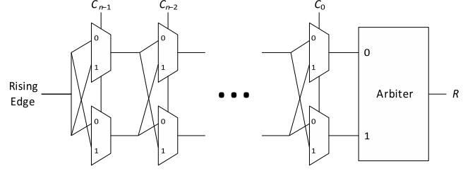
Fig. 1: Standard delay-based arbiter PUF [2].
