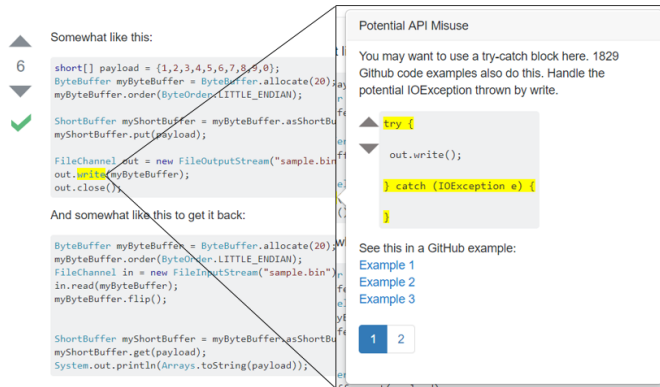
Figure 6: Chrome extension for augmenting Stack Overflow posts with mined API usage
