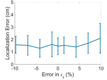
Figure 9— \epsilon_r Variance: For typical variance in human tissue properties, ReMix's localization error continues to be < 2 cm.
