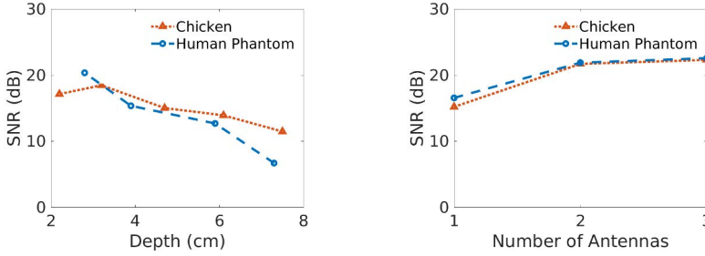
Figure 8—ReMixBackscatter: ReMix can achieve an average SNR of over 15 dB for 1 MHz frequency band even when the tissue depth is up to 8 cm (human muscle depth is 2-3 cm [16]). This SNR can be improved by combining multiple antennas.
