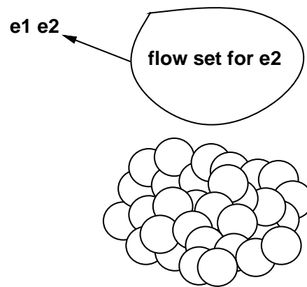
Figure 4: Agesen's analysis.
