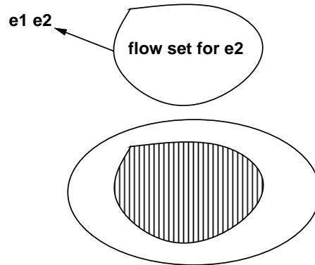
Figure 2: 0-CFA.
