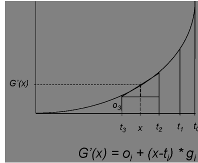
Fig. 2. Gamma correction filter
