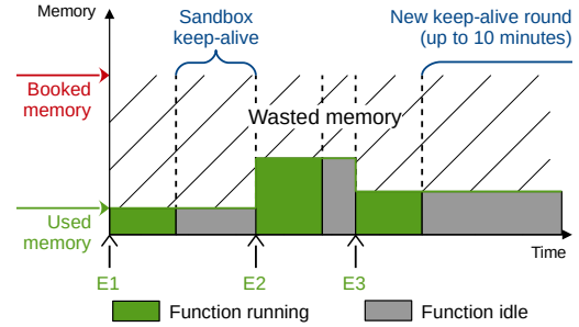
Figure 1. Timeline of a function sandbox with memory waste due to overdimensioning and the keep-alive policy.
