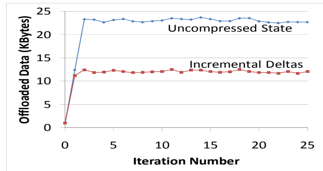
Figure 13: The Performance of the Incremental Deltas to and from the Remote Server. MAUI uses incremental deltas when offloading code to a remote server. In the case of the video game, this optimization reduces the amount of state transferred from 23 KB to 12 KB, on average.
