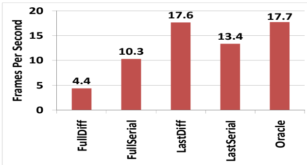
Figure 6: Performance overhead of MAUI profiling. Effect on the game’s performance of five different strategies for the MAUI profiler.
