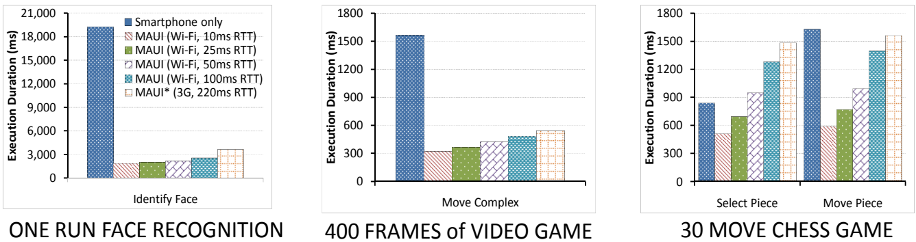
Figure 10: A comparison of MAUI’s performance benefits. We compare the performance of running three application standalone on the smartphone versus using MAUI for remote execution to servers that are successively further away (the RTT is listed for each case). The graph on the left shows one run of the face recognition application; the graph in the middle shows running the video game for 400 frames; the graph on the right shows running the chess game for 30 moves.
