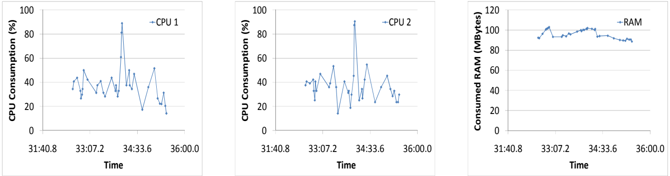
Figure 11: Profiling the Speech Recognition Engine on the MAUI Server. The MAUI server is a 2 GHz Intel Core2 CPU with 2 GB of RAM. The load of one CPU is shown in the graph on the left, whereas the other CPU is shown in the middle. The graph on the right shows the RAM consumed by the speech engine.
