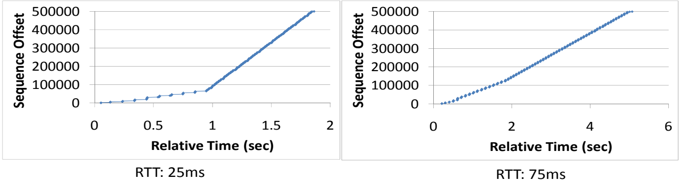
Figure 7: The dynamics of a 500KB TCP transfer with PSM disabled over a two links, one with a 25ms RTT and one with 75ms RTT. During slow-start, for small sender window sizes, the sender goes to sleep after finishing sending its window causing the RTT of the transfer to effectively become 100ms. As the size gets larger, the senders starts receiving TCP ACKs before finishing sending its window worth of segments. The discrepancy between these two regions of a transfer is less pronounced as the link’s RTT increases.
