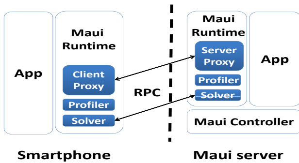
Figure 3: High-level view of MAUI’s architecture.
