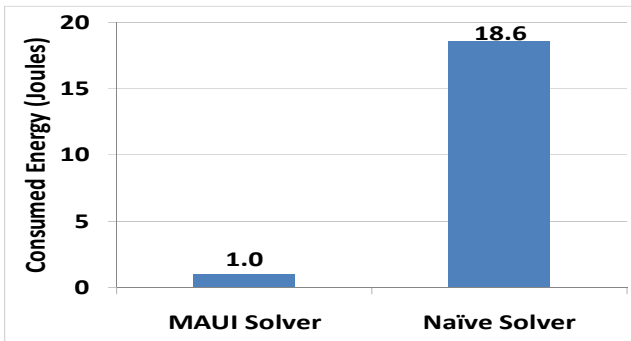
Figure 12: The energy consumed by the face recognition application for different code offload solvers. We ran the application using both the MAUI solver and a naïve solver takes a local view of the program.
