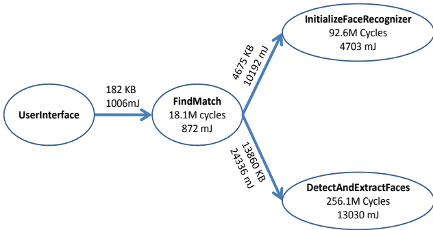
Figure 8: The call graph of a face recognition application. Each vertex represents a method and its computational and energy costs, and each edge represents the size of the method’s state and the energy consumed to transfer this state remotely.
