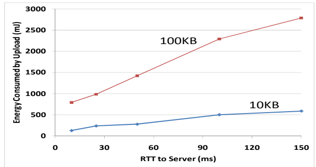
Figure 2: The Energy Consumed by Offloading 10 KB and 100 KB of Code to the Cloud for Various Round-Trip Times to the Server. We used power-save mode (PSM) for the results presented in this graph; we also conducted experiment with no PSM that show the same trends. High RTTs lead to significant increases in the energy consumption.
