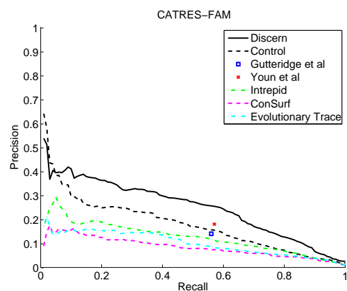
Fig. 2. Results on the CATRES-FAM benchmark dataset. Methods included in this analysis are a neural-network method from Gutteridge and colleagues (Gutteridge et al. , 2003), a Support Vector Machine approach from Youn and colleagues (Youn et al. , 2007), ConSurf (Landau et al. , 2005), INTREPID (Sankararaman and Sjölander, 2008), Evolutionary Trace (Mihalek et al. , 2004) and the control method described in Table 1. The methods of Youn et al. , Gutteridge et al. , and the control use information from both sequence and structure, while ConSurf, INTREPID and Evolutionary Trace use conservation signal only to predict catalytic sites. In cross-validation experiments on this dataset, at 18% precision, DISCERN reaches 69% recall, corresponding to a gain in recall of 20% over Gutteridge et al. and 12% over Youn et al. (based on their reported performance at this level of precision on similar datasets). Relative to the methods that use conservation signal only, the difference is greater: at 18% precision, INTREPID reaches 19% recall while Evolutionary Trace reaches a recall of 2%. ConSurf does not reach 18% precision on this dataset.
