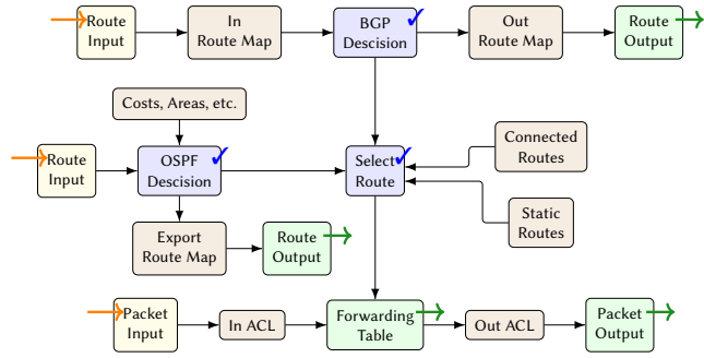
Figure 4: Basic features of routing and forwarding. Blue nodes (✓) represent fixed processes. Yellow nodes (incoming →) are inputs and green nodes (outgoing →) are outputs. Unmarked (brown) nodes represent configurable entities.
