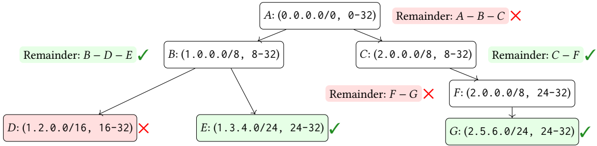
Figure 3: DAG created from prefix ranges. Green (✓) nodes represent leaves or remainders contained in a set S , and red (✗) nodes represent those that are not. S can be represented by the union of B - D - E , C - F , and G
