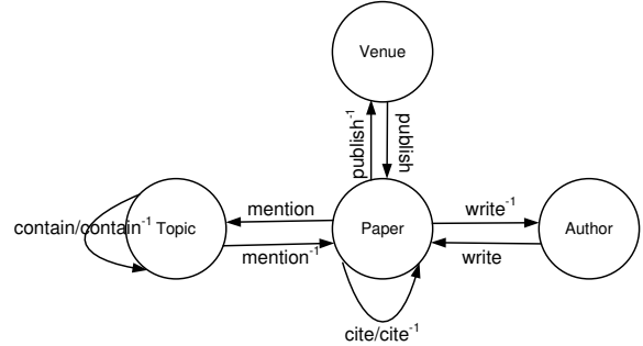
Figure 1. Schema for DBLP Bibliographic Network
