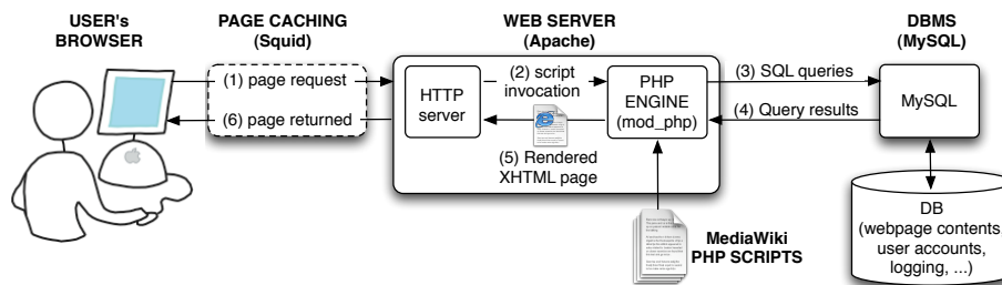
Figure 1: MediaWiki Software Architecture
