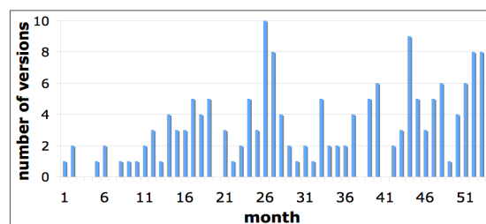
Figure 6: Schema Versions Committed during Each Month
