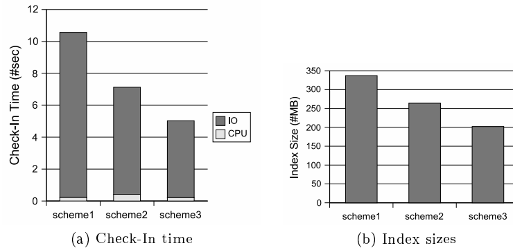
Fig. 6. Comparing the check-in time and the index sizes.
