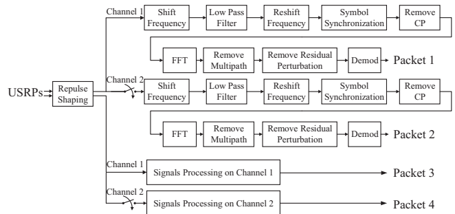
Fig. 5. Receiving chain
