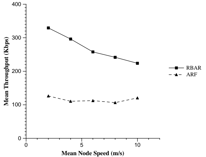
Figure 19: Performance comparison for a single CBR connection in a multihop network.
