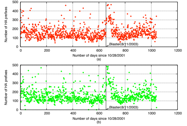
Fig. 3. (a) Number of HA prefixes per day, from monitor 144.228.241.81 and (b) with offset of 12h in day slot.
