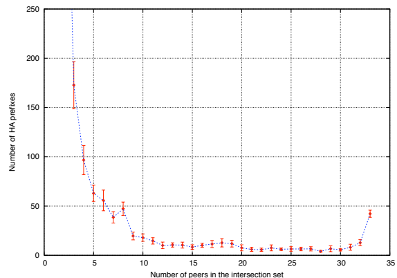
Fig. 7. HA prefix intersection over 33 different peers, May 2004
