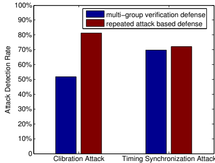
Fig. 7: Attack detection rate of the two defenses.
