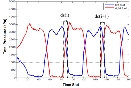
Fig. 3: The waveform of the double support metric.
