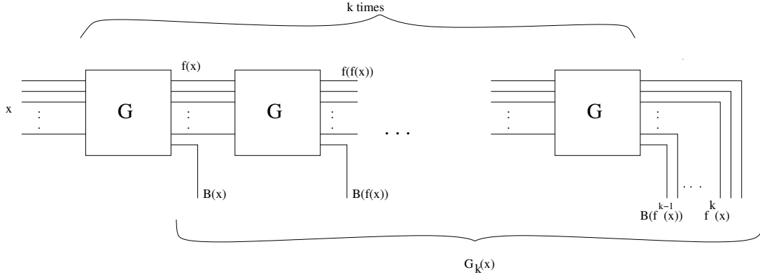
Figure 13.1: Pseudorandom generator
