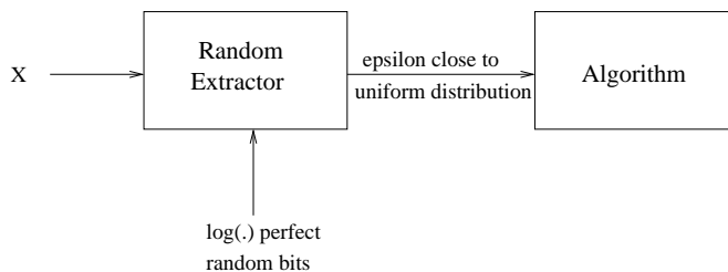
Figure 27.3: Random Extractors
