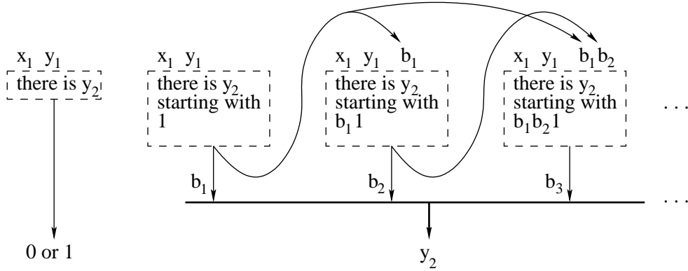
Figure 6.6: How to use decision problem solvers to find a witness to a search problem.
