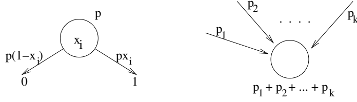
Figure 8.2: Constructing the polynomial of a branching program.
