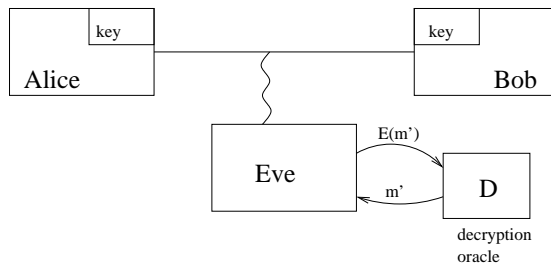
Figure 13.6: Stronger threat model
