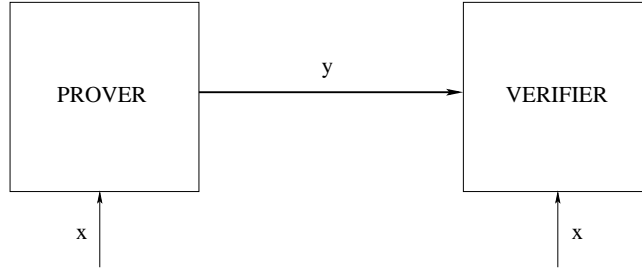
Figure 17.1: NP with a Prover-Verifier mechanism
