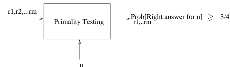
Figure 27.1: Ideal probabilistic algorithm
